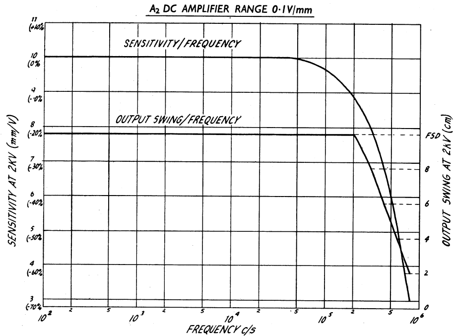
Fig. 3 Response Curve for A 2 Amplifier
